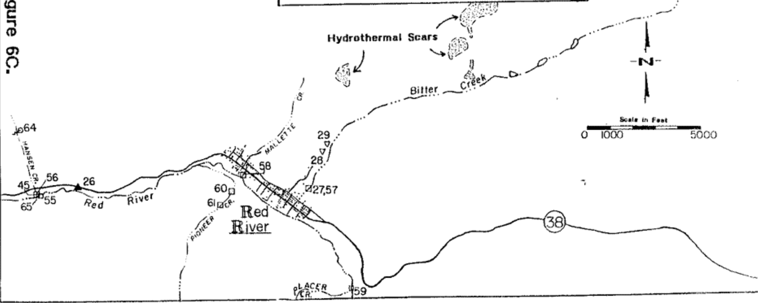
Figure 6C. Location of sample sites for the Red River ground water investigation. East panel, number 3 of 3 segments (see inset map); analytical data and description of site compiled in Table 1 . EXPLANATION ○ Seep / Spring Samples ● Mine Area Monitor Wells ⊙ Mill Tailings Piles Monitor Wells ▽ Private Well ▲ Public Well E Extraction Well □ Stream Sample
