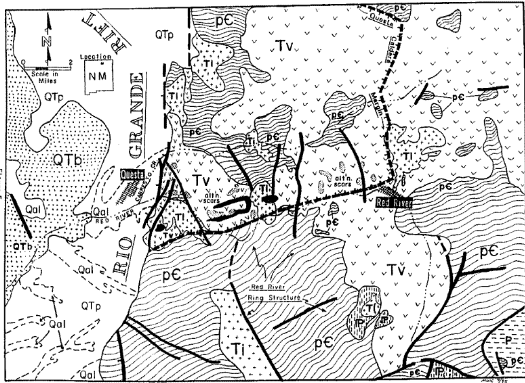
Figure 5. Composite Geologic Map of Red River-Questa Area.
